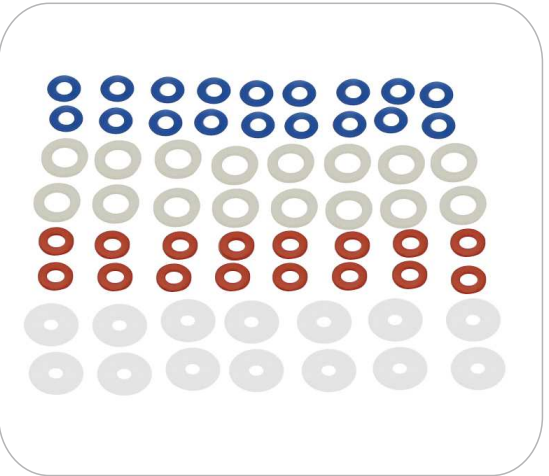
材质：聚酯（PET） 内径:最小0.5mm 外径：可按客户要求定制 厚度：0.05mm-0.5mm Material: polyester (PET) Inside diameter: minimum 0.5mm External diameter: can be customized according to customer requirements Thickness: 0.05mm-0.5mm
