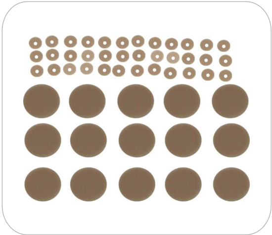
材质：PEEK 内径:最小0.6mm 外径：可按客户要求定制 厚度：0.05mm-1.0mm Material: PEEK Inside diameter: minimum 0.6mm External diameter: can be customized according to customer requirements Thickness: 0.05mm-1.0mm
